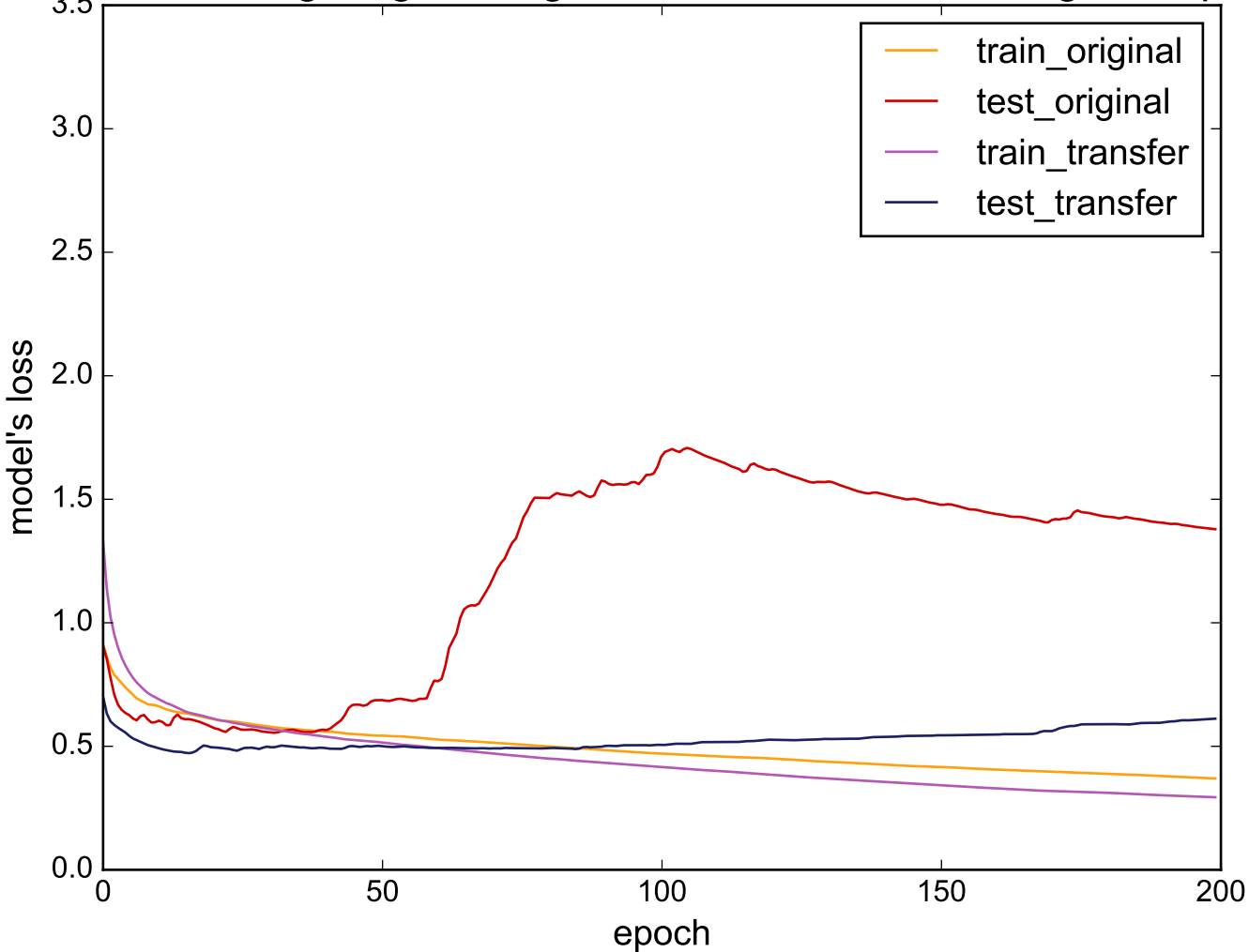
Source: Lighting2 - Target: DistalPhalanxOutlineAgeGroup
