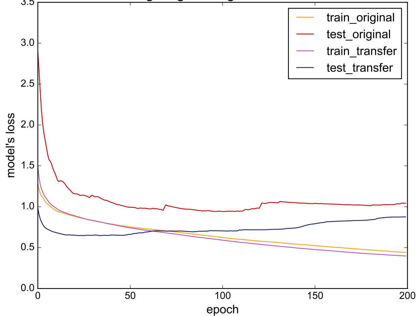
Source: Lighting2 - Target: DistalPhalanxTW
