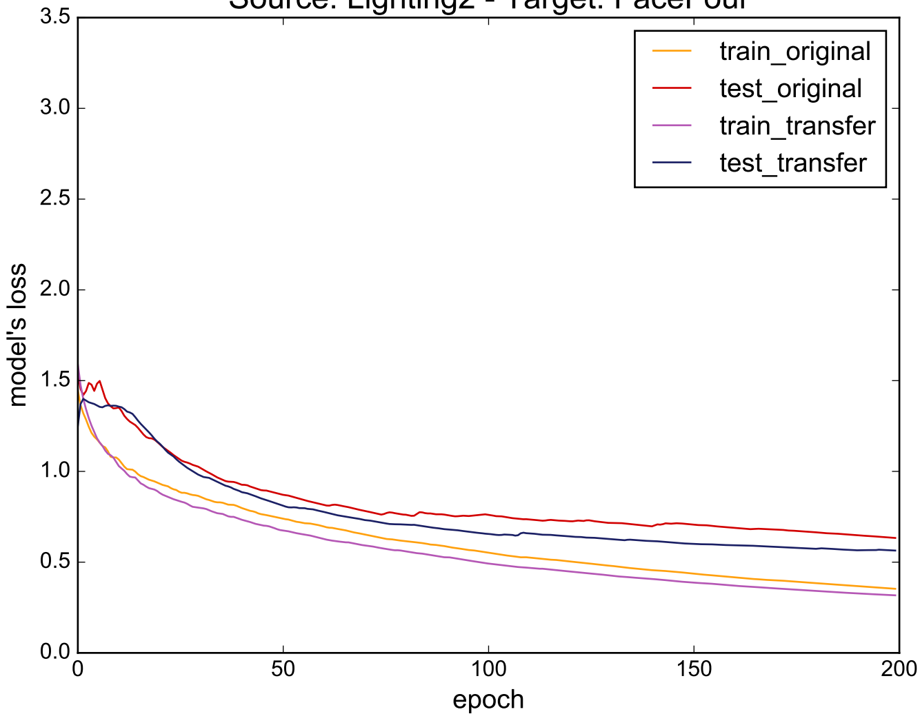
Source: Lighting2 - Target: FaceFour
