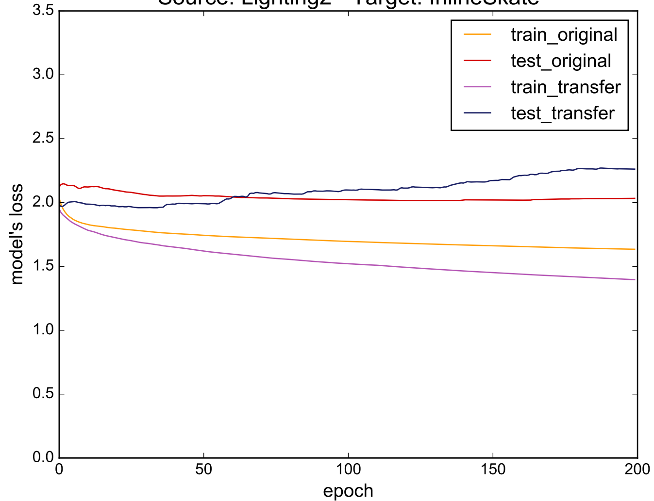
Source: Lighting2 - Target: InlineSkate
