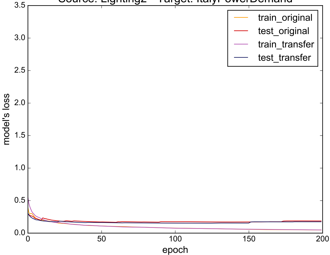
Source: Lighting2 - Target: ItalyPowerDemand
