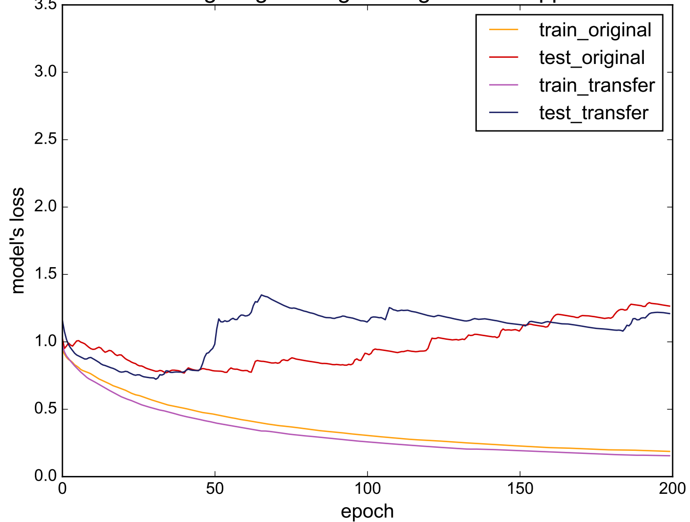
Source: Lighting2 - Target: LargeKitchenAppliances
