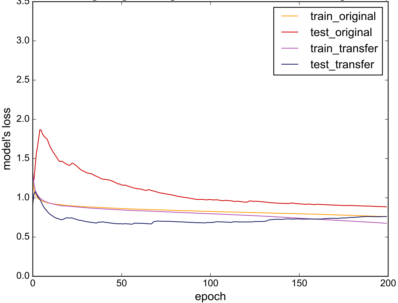
Source: Lighting2 - Target: MiddlePhalanxOutlineAgeGroup
