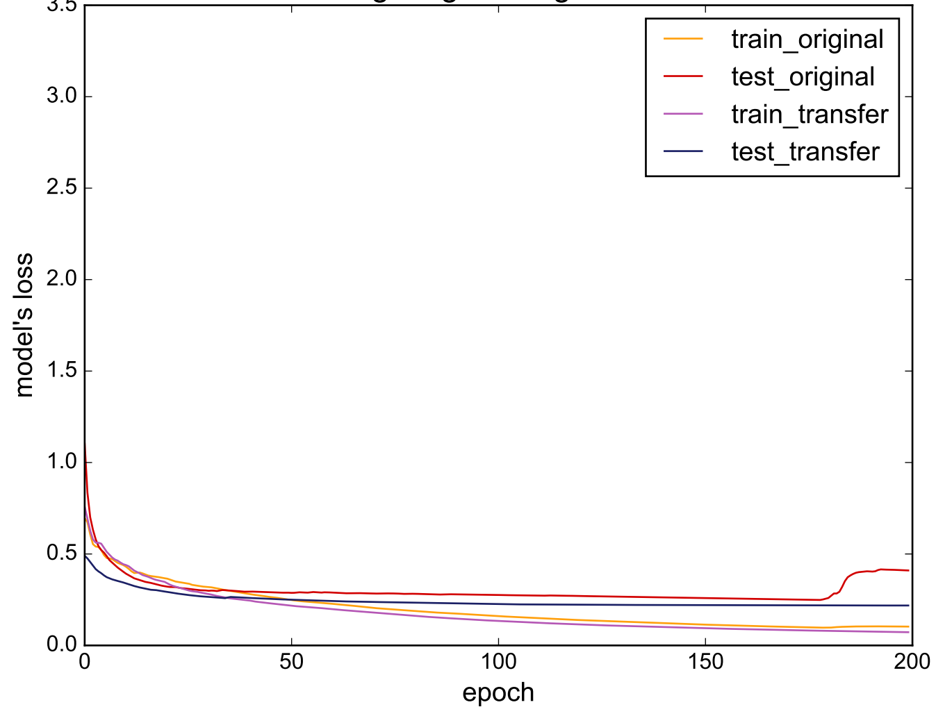
Source: Lighting2 - Target: MoteStrain
