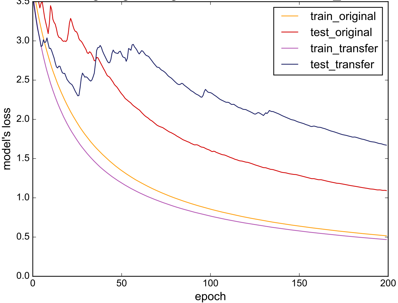
Source: Lighting2 - Target: NonInvasiveFetalECG_Thorax1
