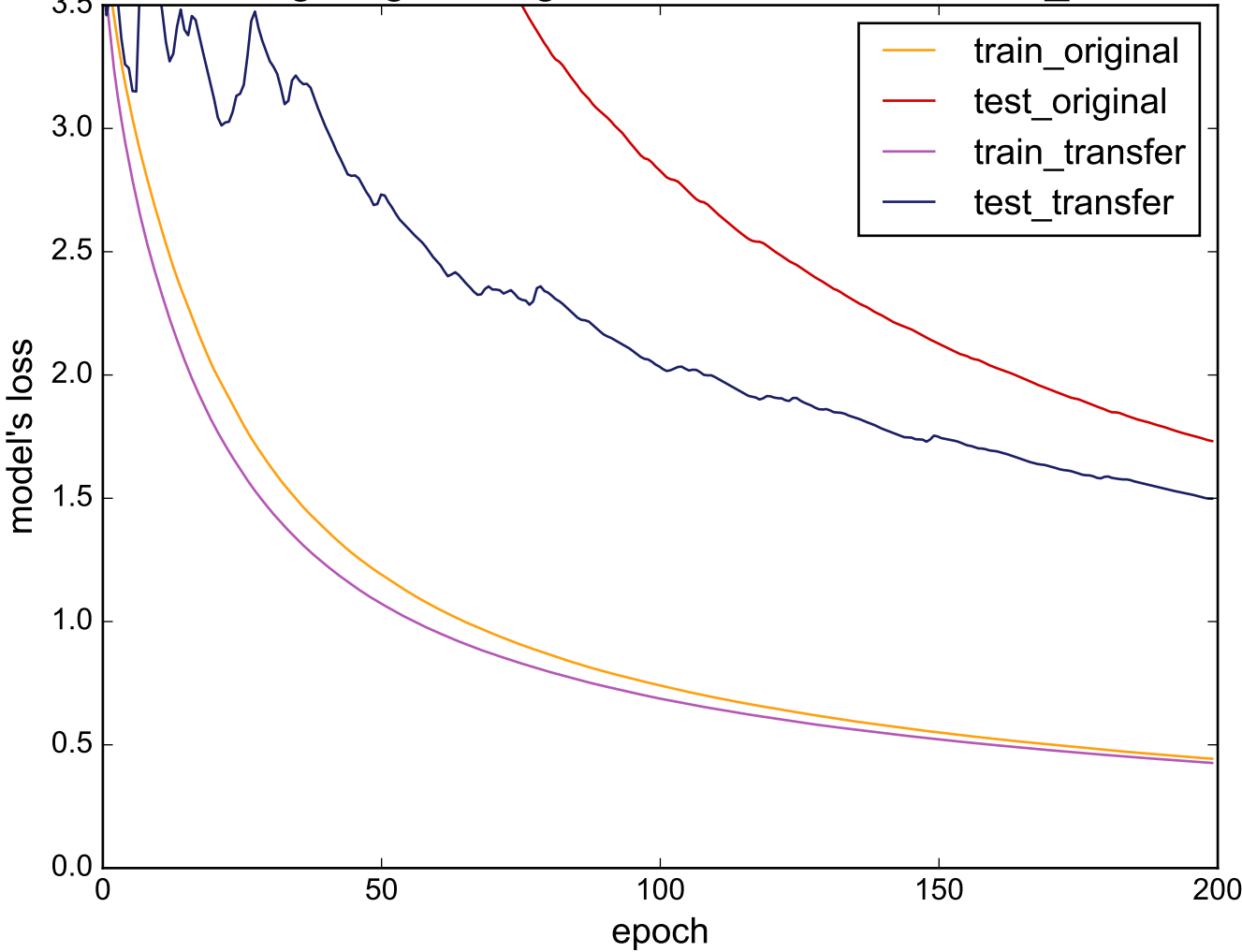
Source: Lighting2 - Target: NonInvasiveFetalECG_Thorax2
