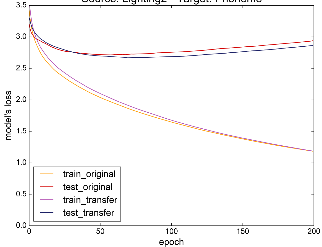
Source: Lighting2 - Target: Phoneme
