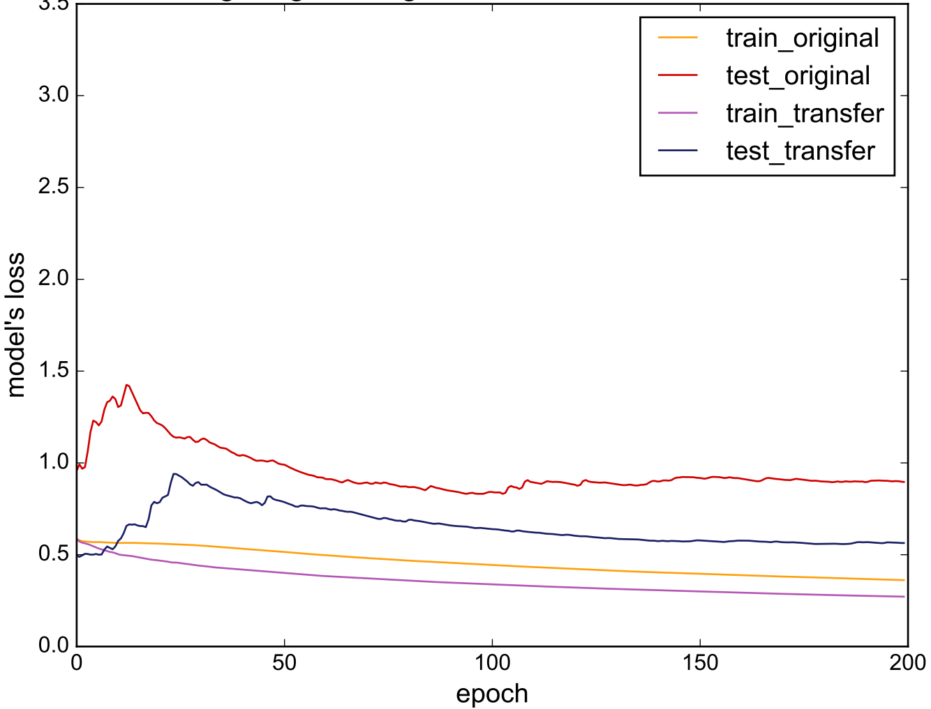
Source: Lighting2 - Target: ProximalPhalanxOutlineCorrect
