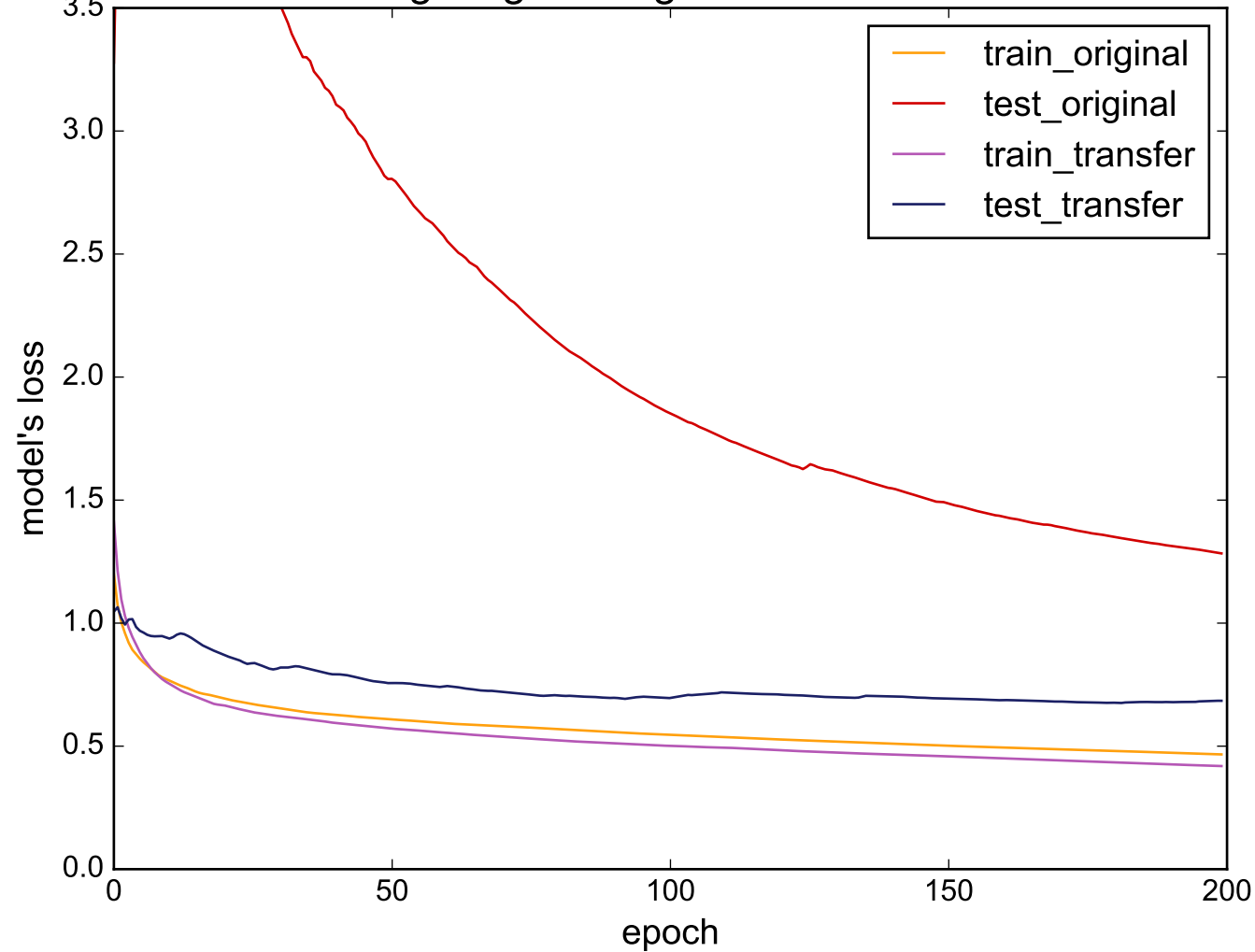
Source: Lighting2 - Target: ProximalPhalanxTW
