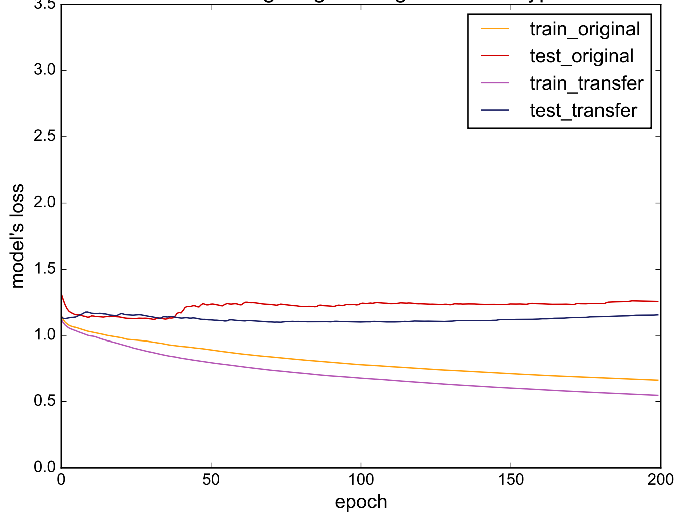
Source: Lighting2 - Target: ScreenType
