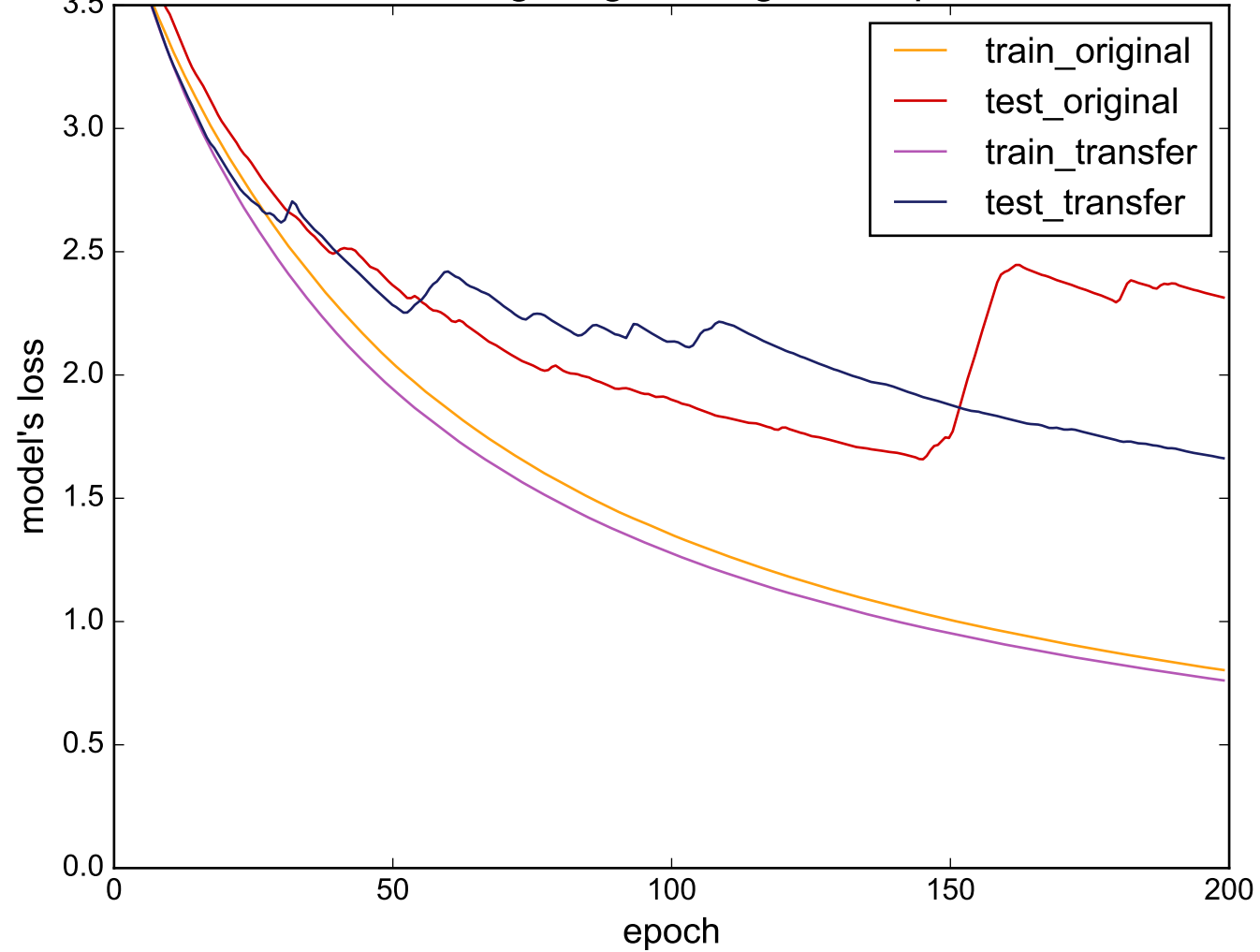
Source: Lighting2 - Target: ShapesAll
