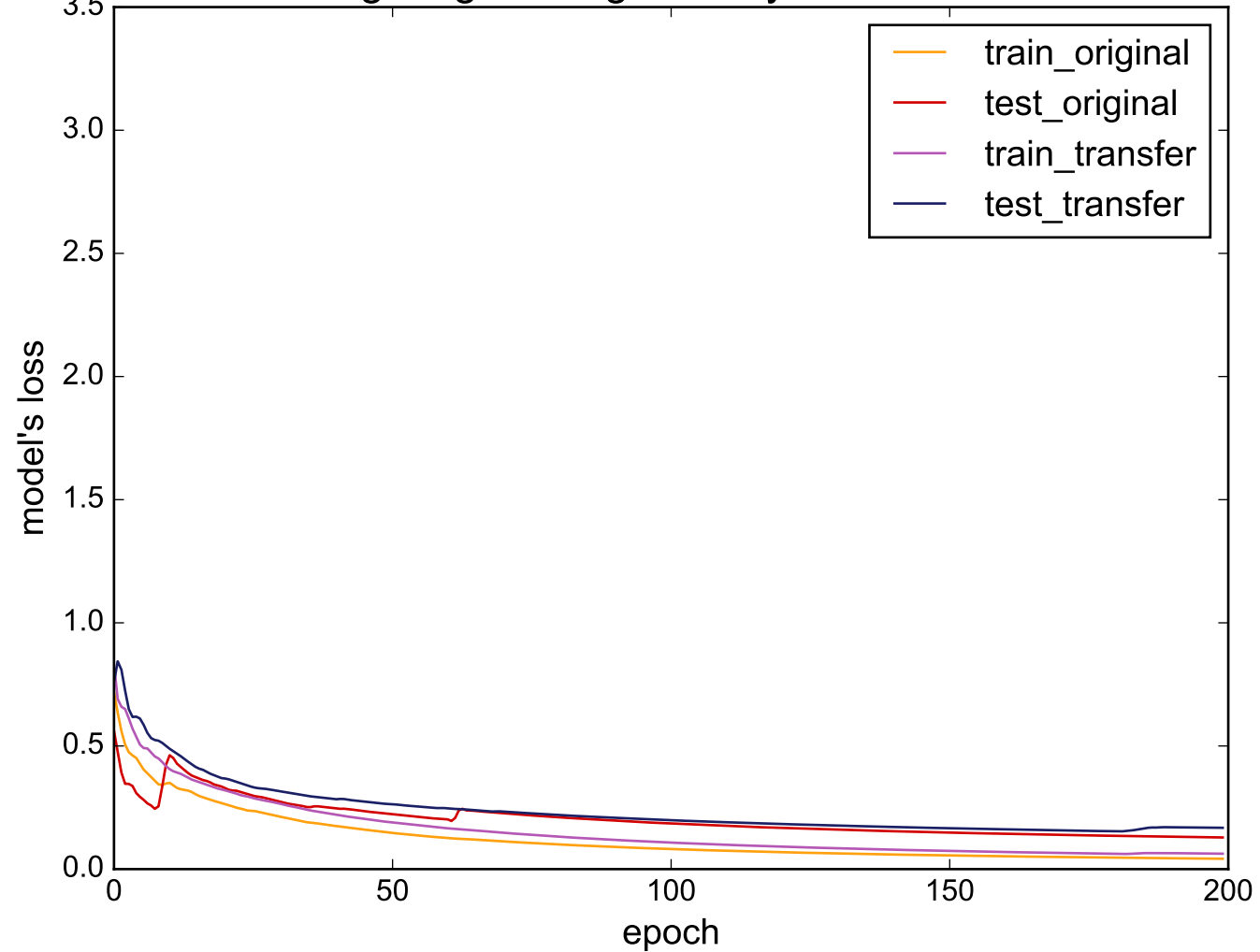
Source: Lighting2 - Target: SonyAIBORobotSurfaceII
