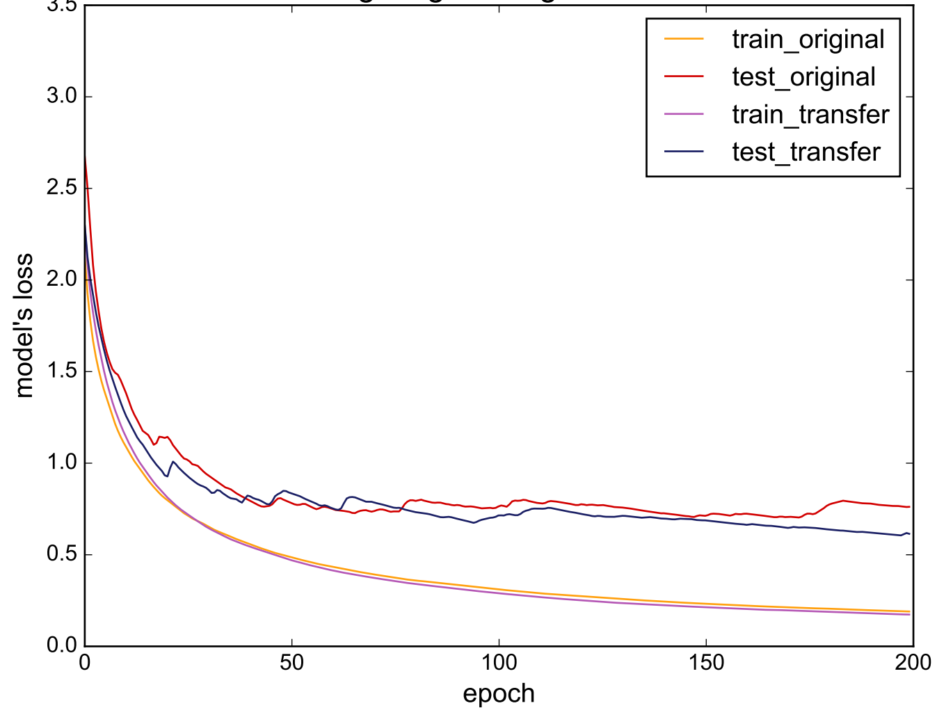
Source: Lighting2 - Target: SwedishLeaf
