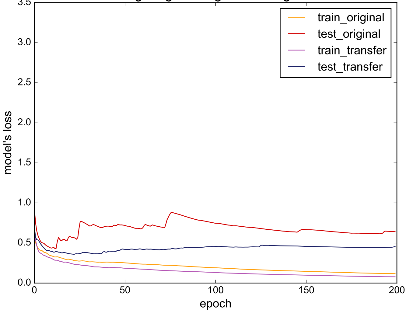
Source: Lighting2 - Target: ToeSegmentation2
