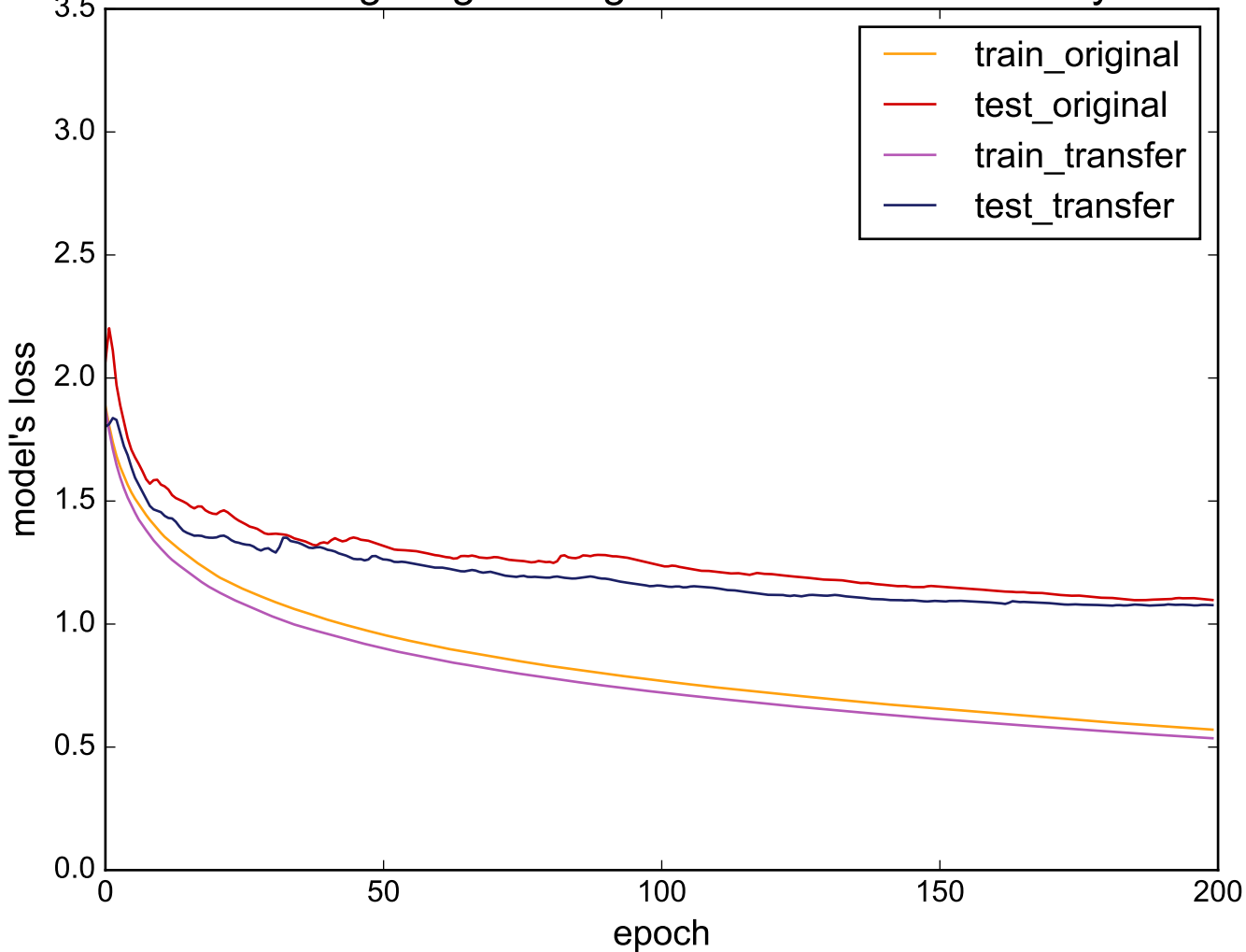
Source: Lighting2 - Target: UWaveGestureLibraryAll
