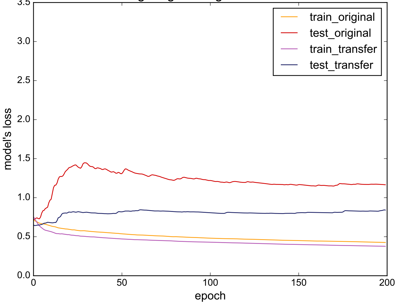
Source: Lighting2 - Target: WormsTwoClass
