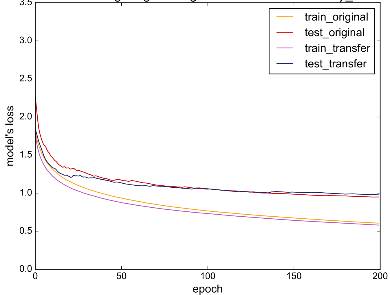
Source: Lighting2 - Target: uWaveGestureLibrary_X
