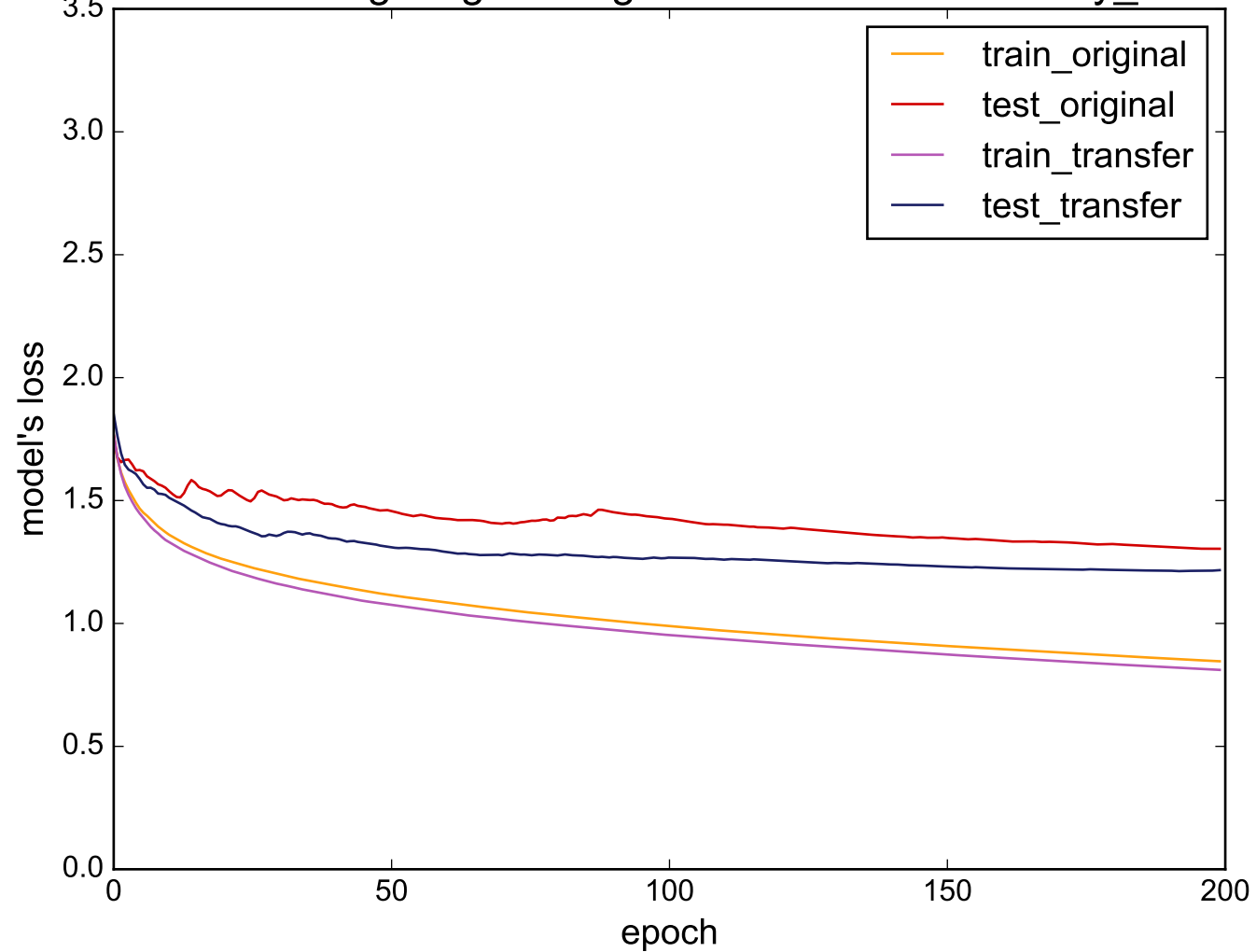
Source: Lighting2 - Target: uWaveGestureLibrary_Y
