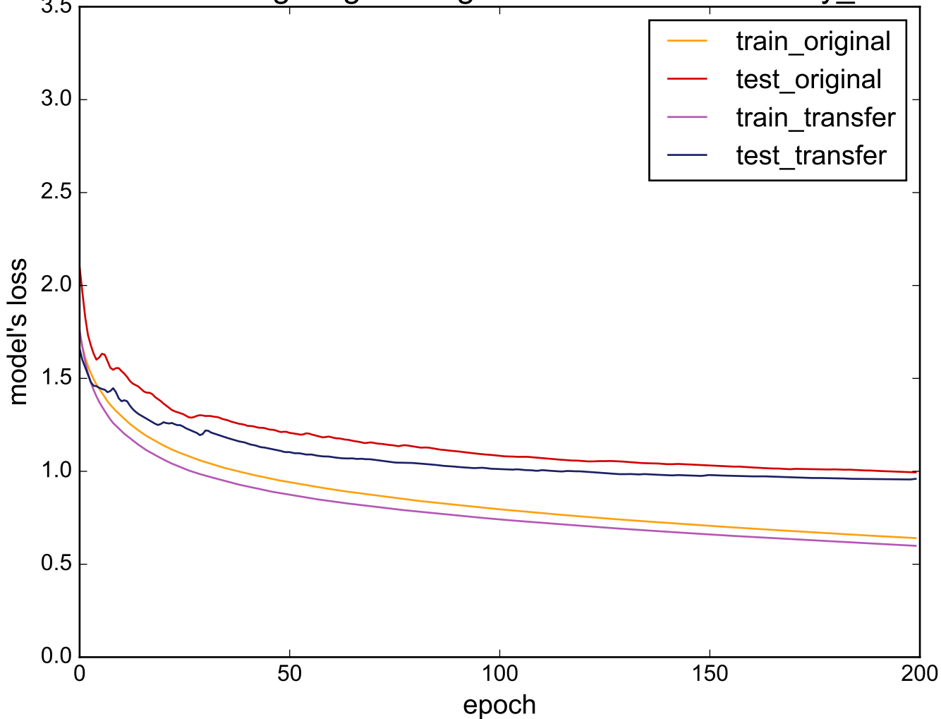
Source: Lighting2 - Target: uWaveGestureLibrary_Z
