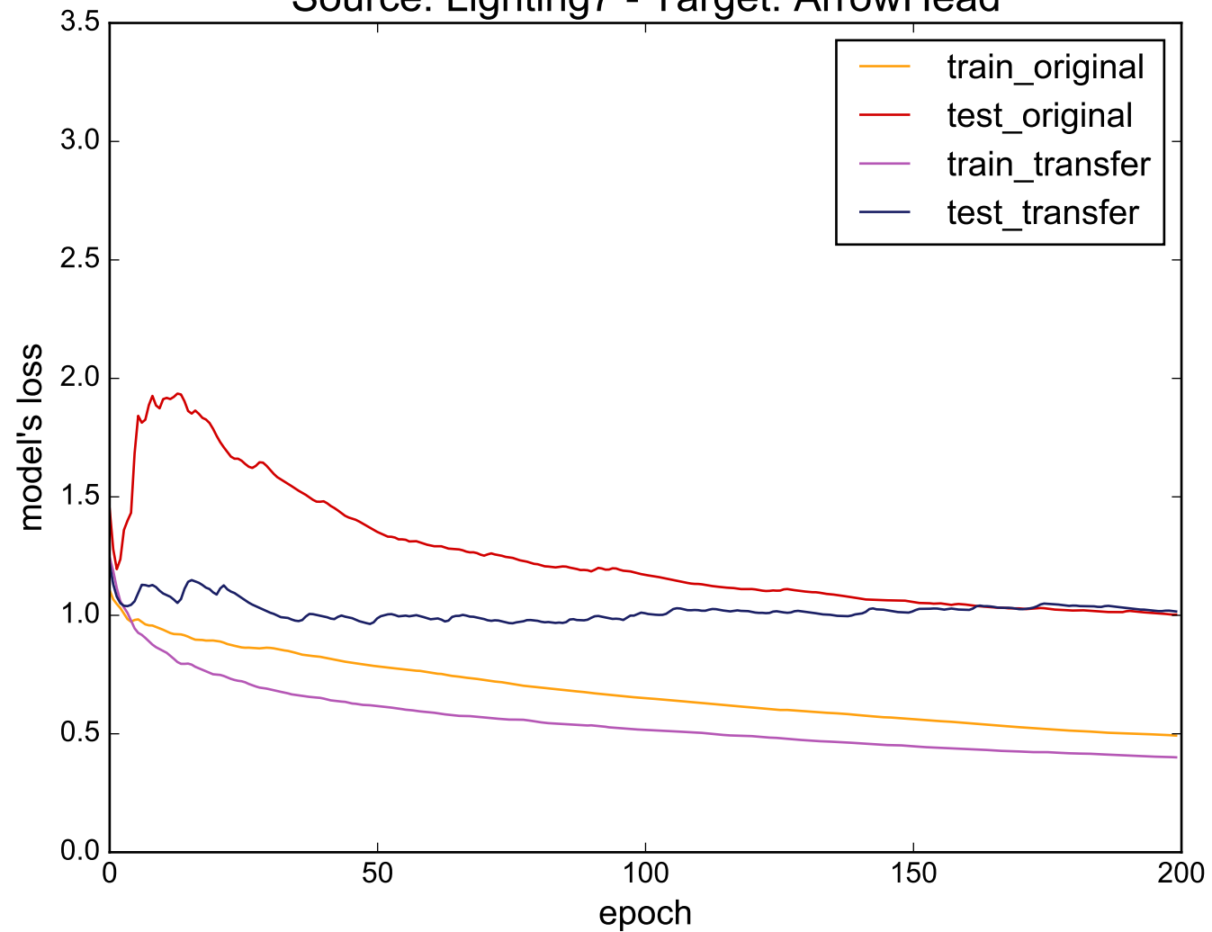
Source: Lighting7 - Target: ArrowHead
