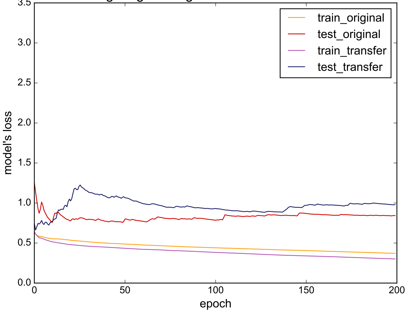
Source: Lighting7 - Target: DistalPhalanxOutlineCorrect
