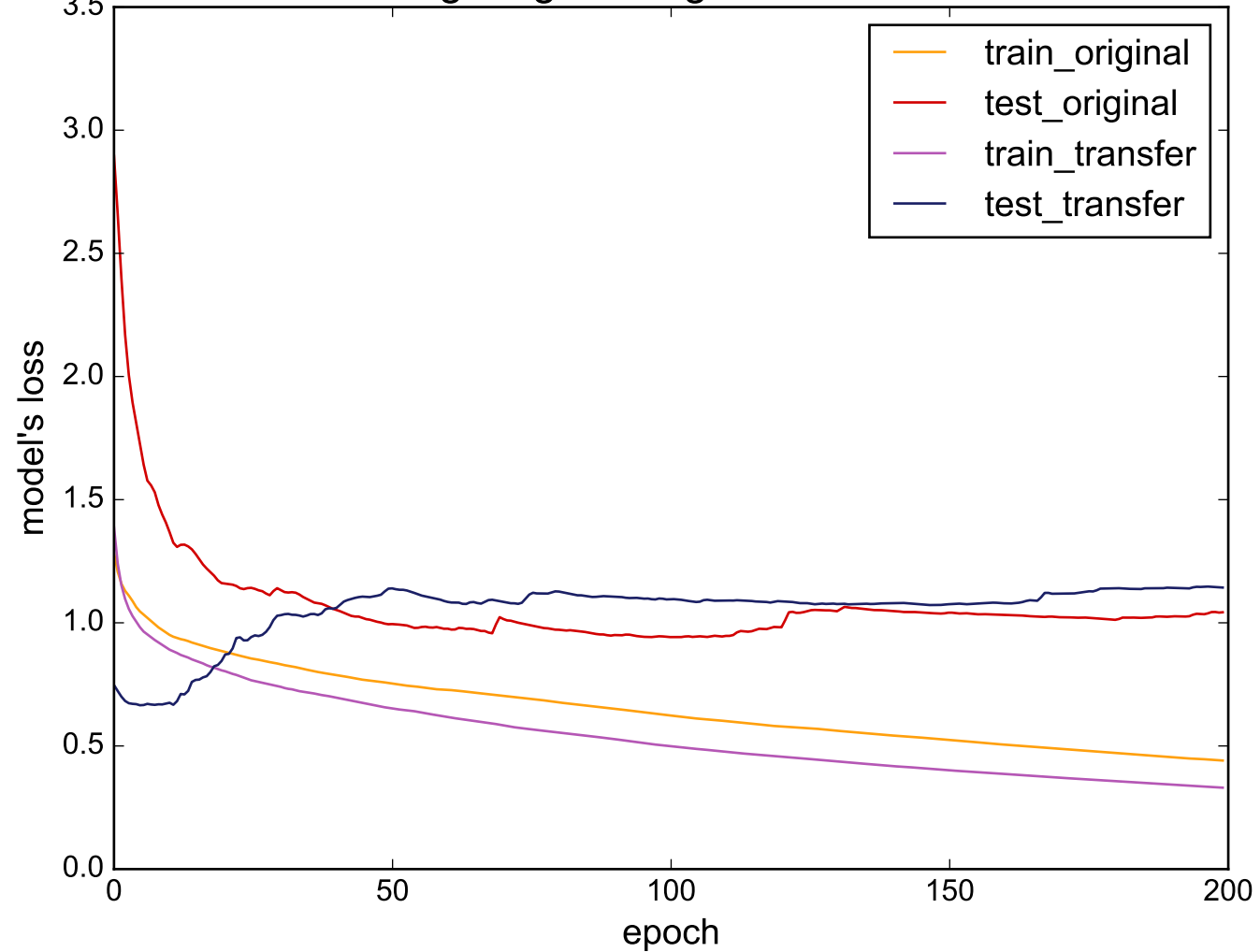
Source: Lighting7 - Target: DistalPhalanxTW
