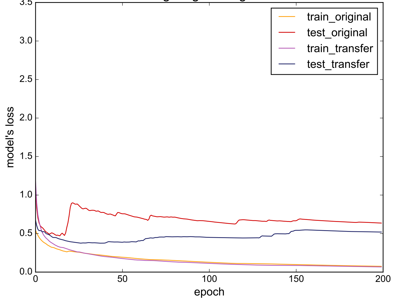
Source: Lighting7 - Target: ECG200
