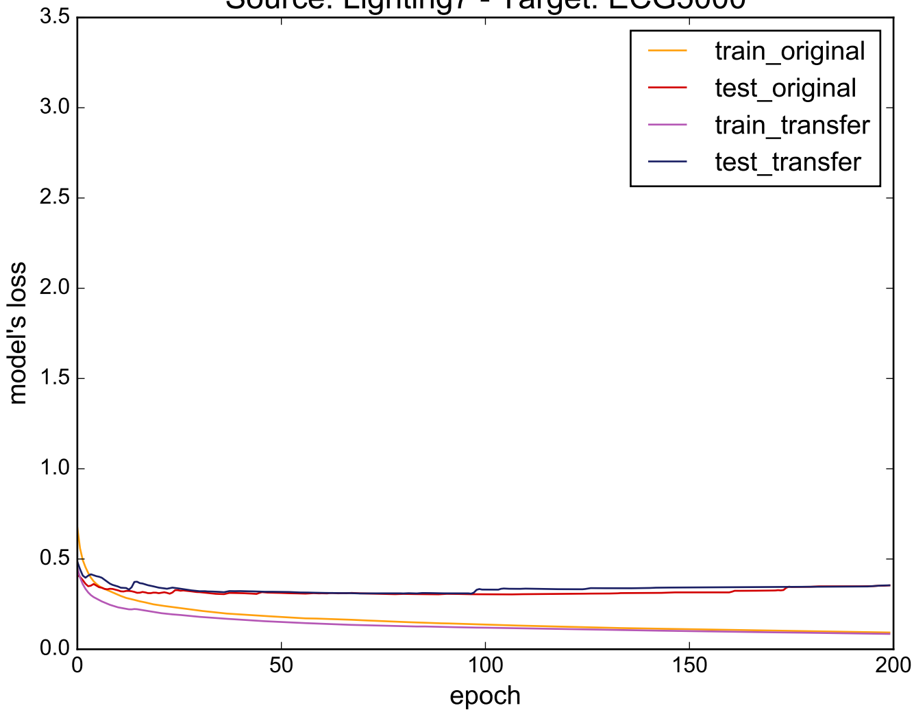
Source: Lighting7 - Target: ECG5000
