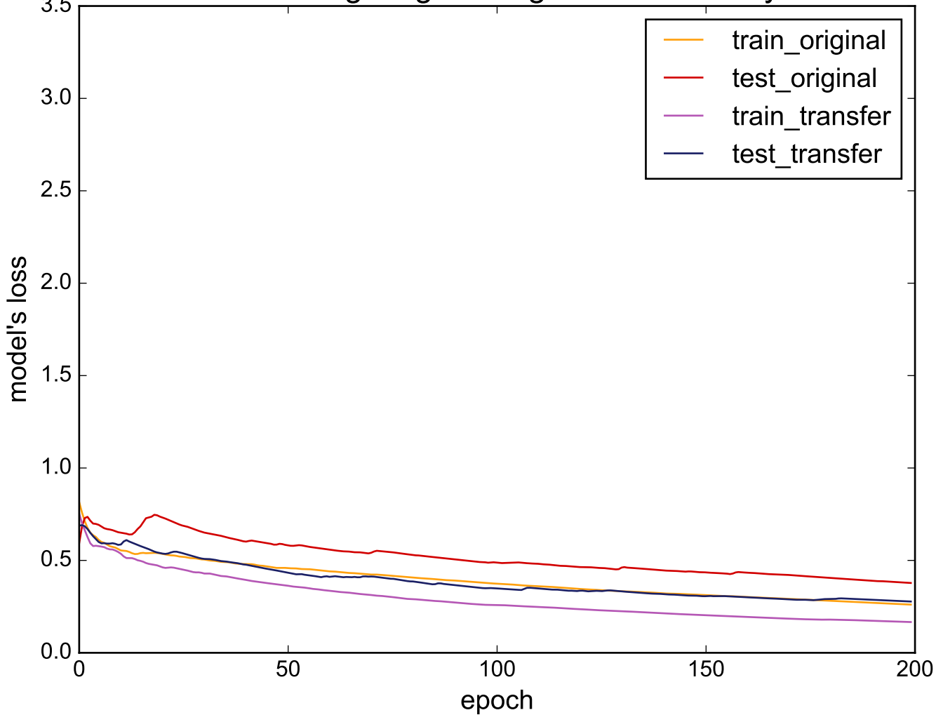
Source: Lighting7 - Target: ECGFiveDays
