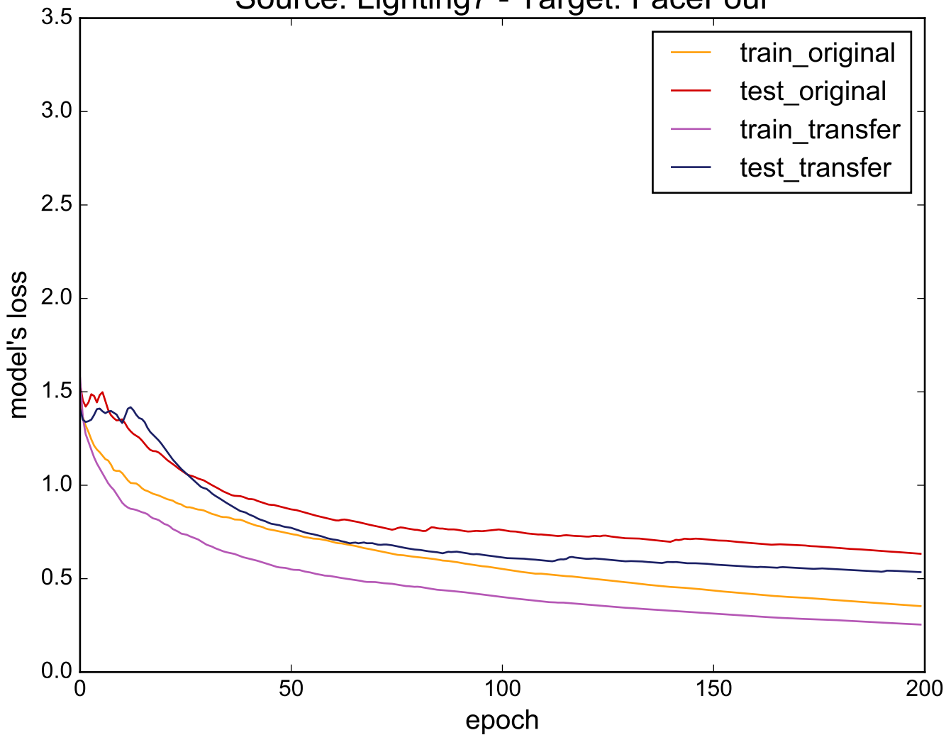
Source: Lighting7 - Target: FaceFour
