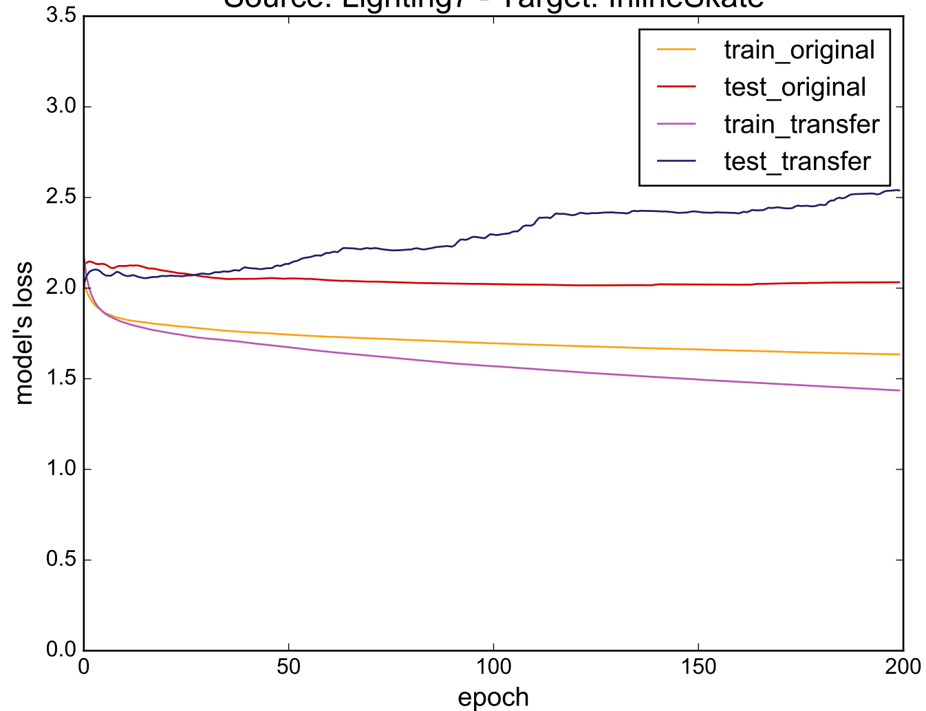
Source: Lighting7 - Target: InlineSkate
