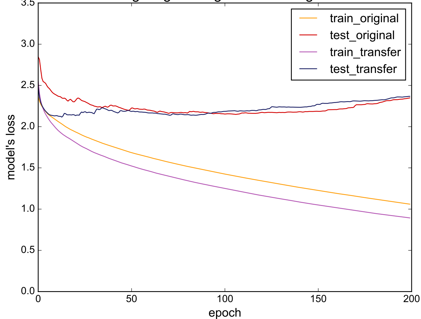
Source: Lighting7 - Target: InsectWingbeatSound
