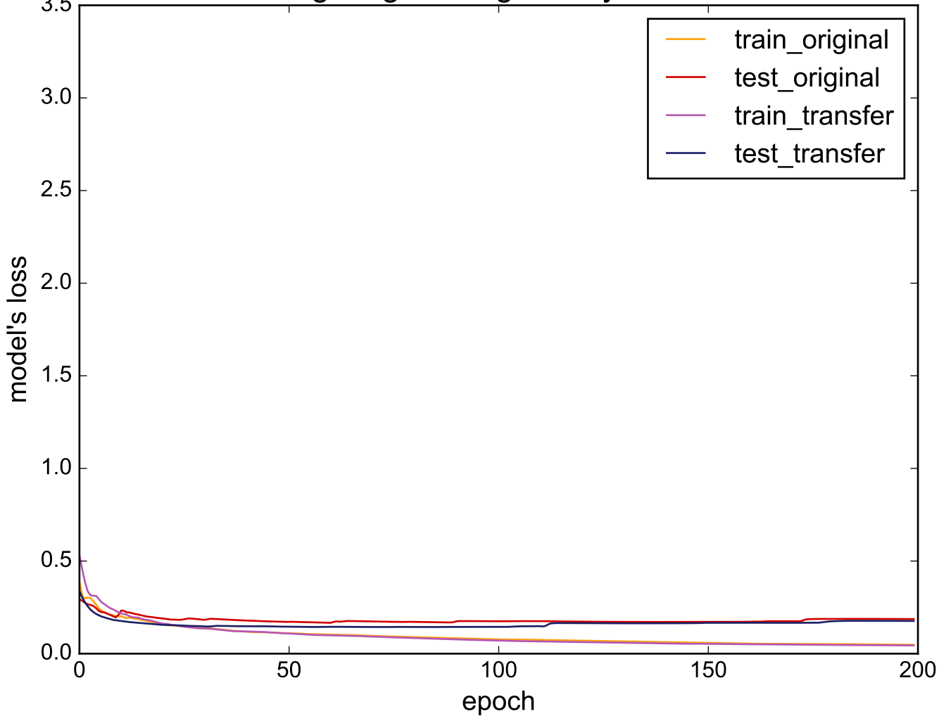
Source: Lighting7 - Target: ItalyPowerDemand
