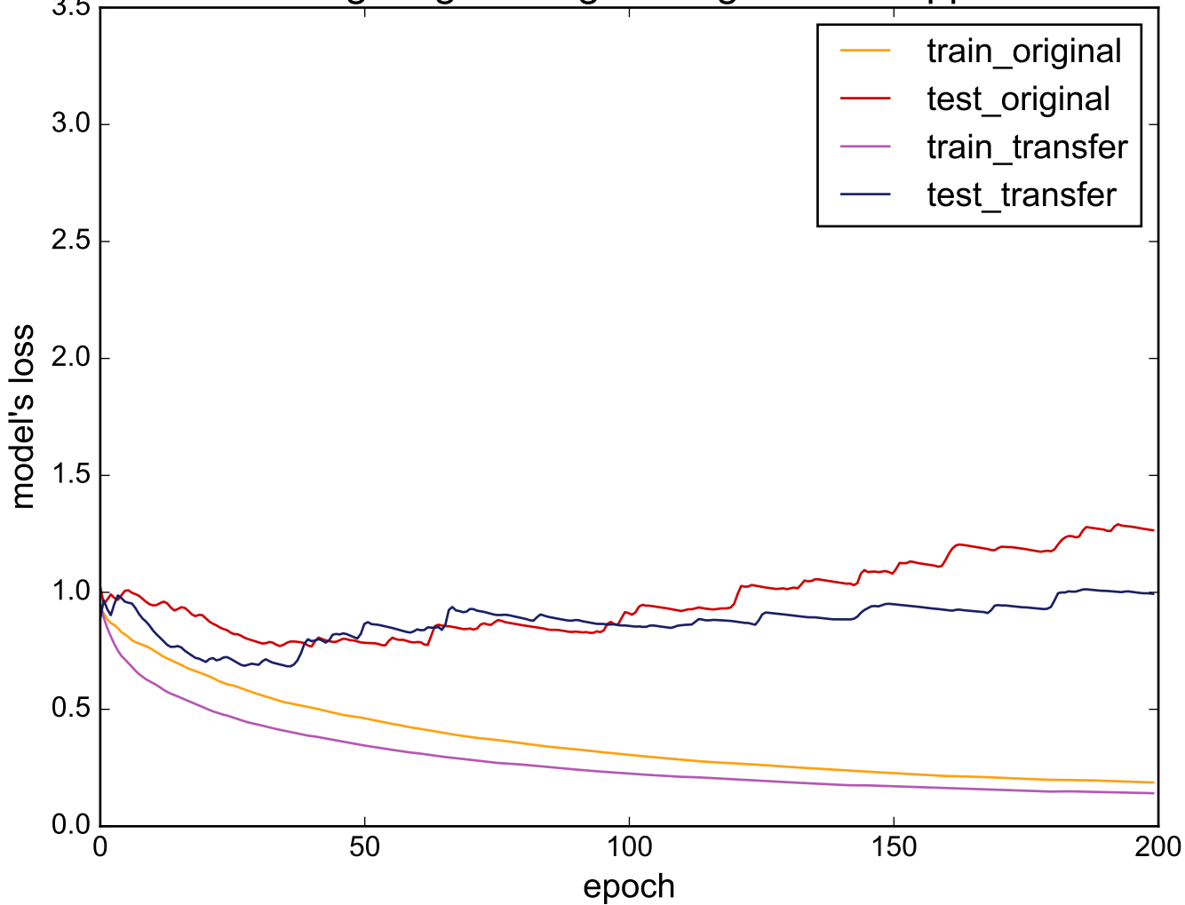
Source: Lighting7 - Target: LargeKitchenAppliances
