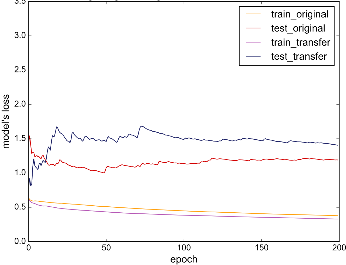
Source: Lighting7 - Target: MiddlePhalanxOutlineCorrect
