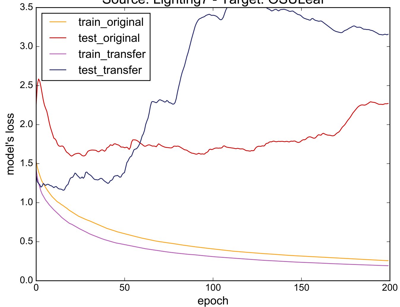
Source: Lighting7 - Target: OSULeaf
