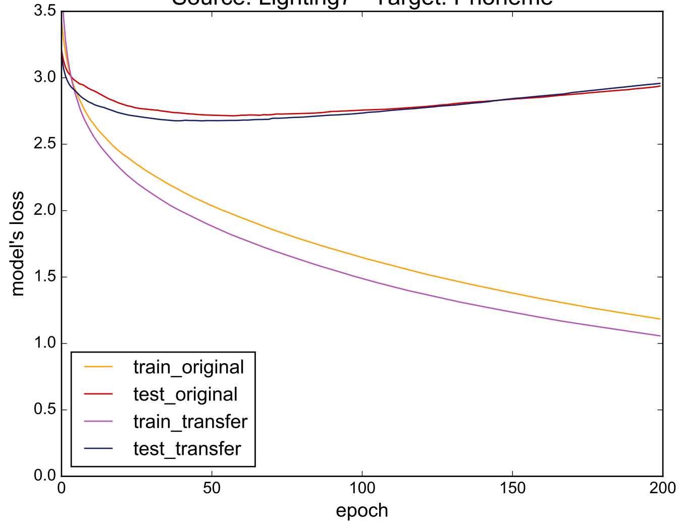
Source: Lighting7 - Target: Phoneme
