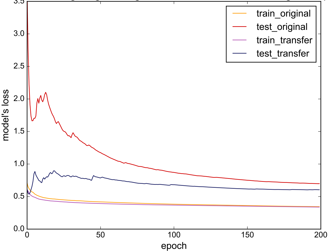
Source: Lighting7 - Target: ProximalPhalanxOutlineAgeGroup
