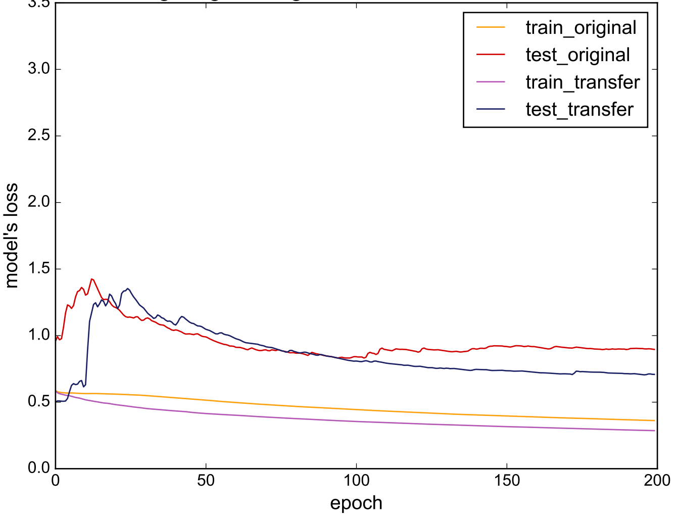
Source: Lighting7 - Target: ProximalPhalanxOutlineCorrect
