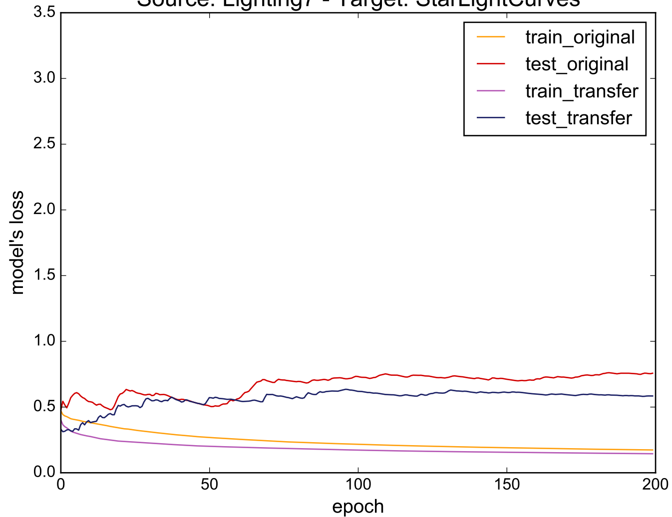
Source: Lighting7 - Target: StarLightCurves
