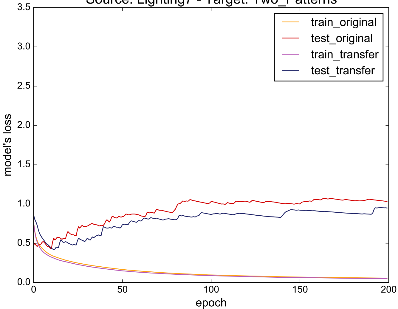
Source: Lighting7 - Target: Two_Patterns
