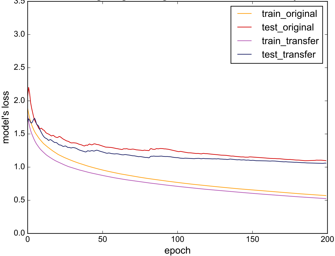
Source: Lighting7 - Target: UWaveGestureLibraryAll
