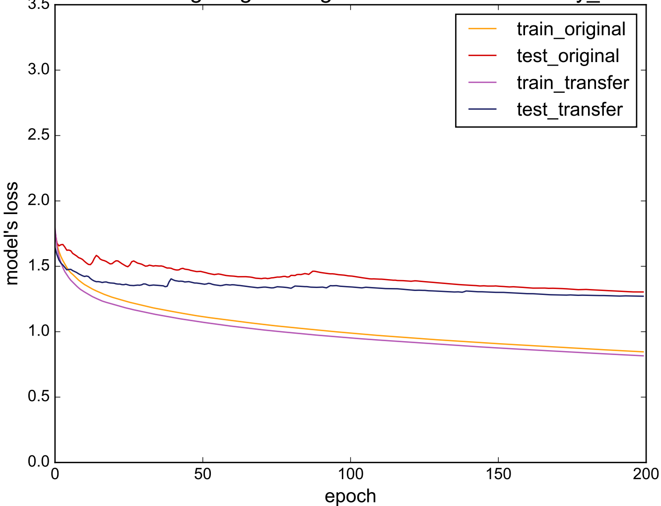
Source: Lighting7 - Target: uWaveGestureLibrary_Y
