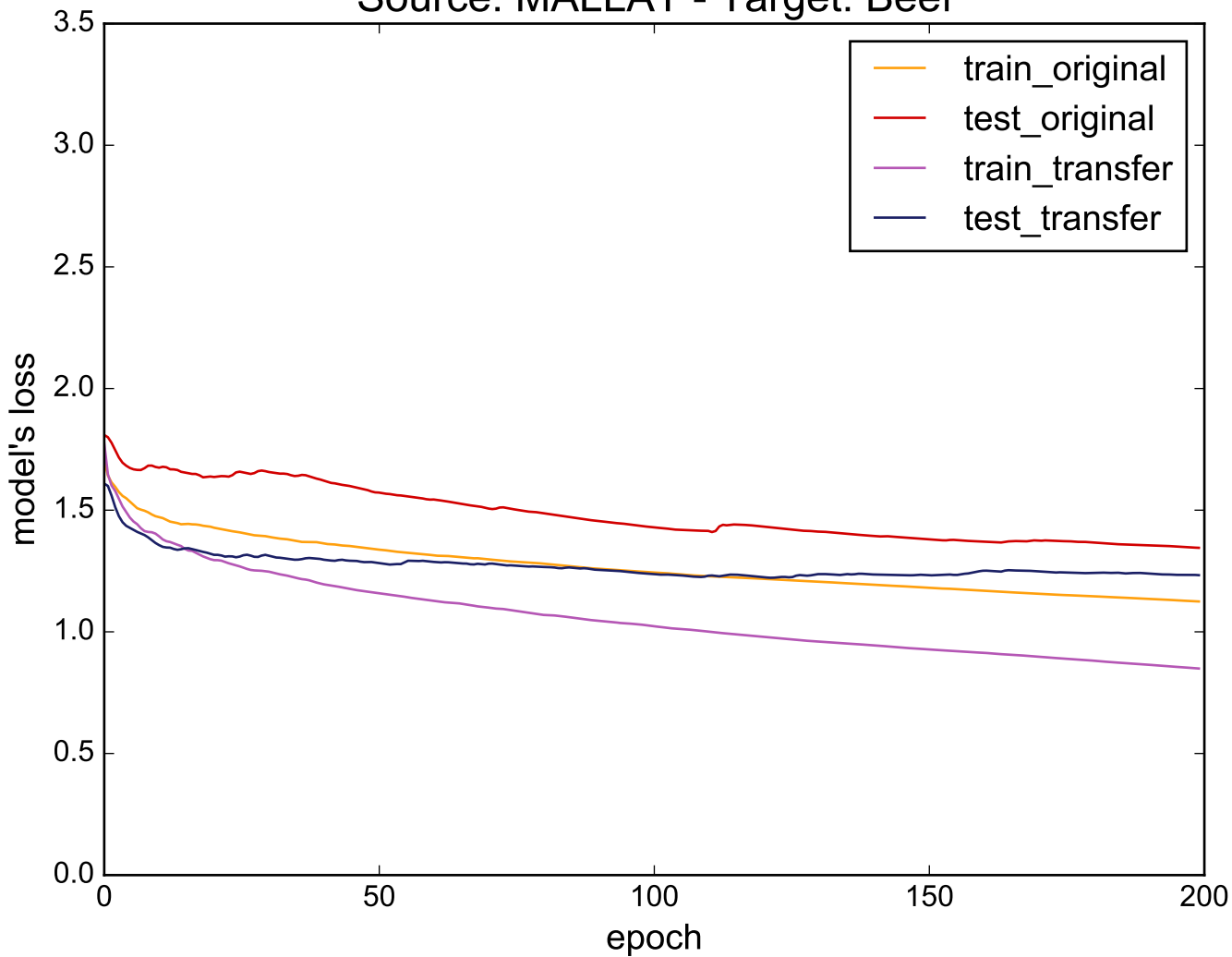
Source: MALLAT - Target: Beef
