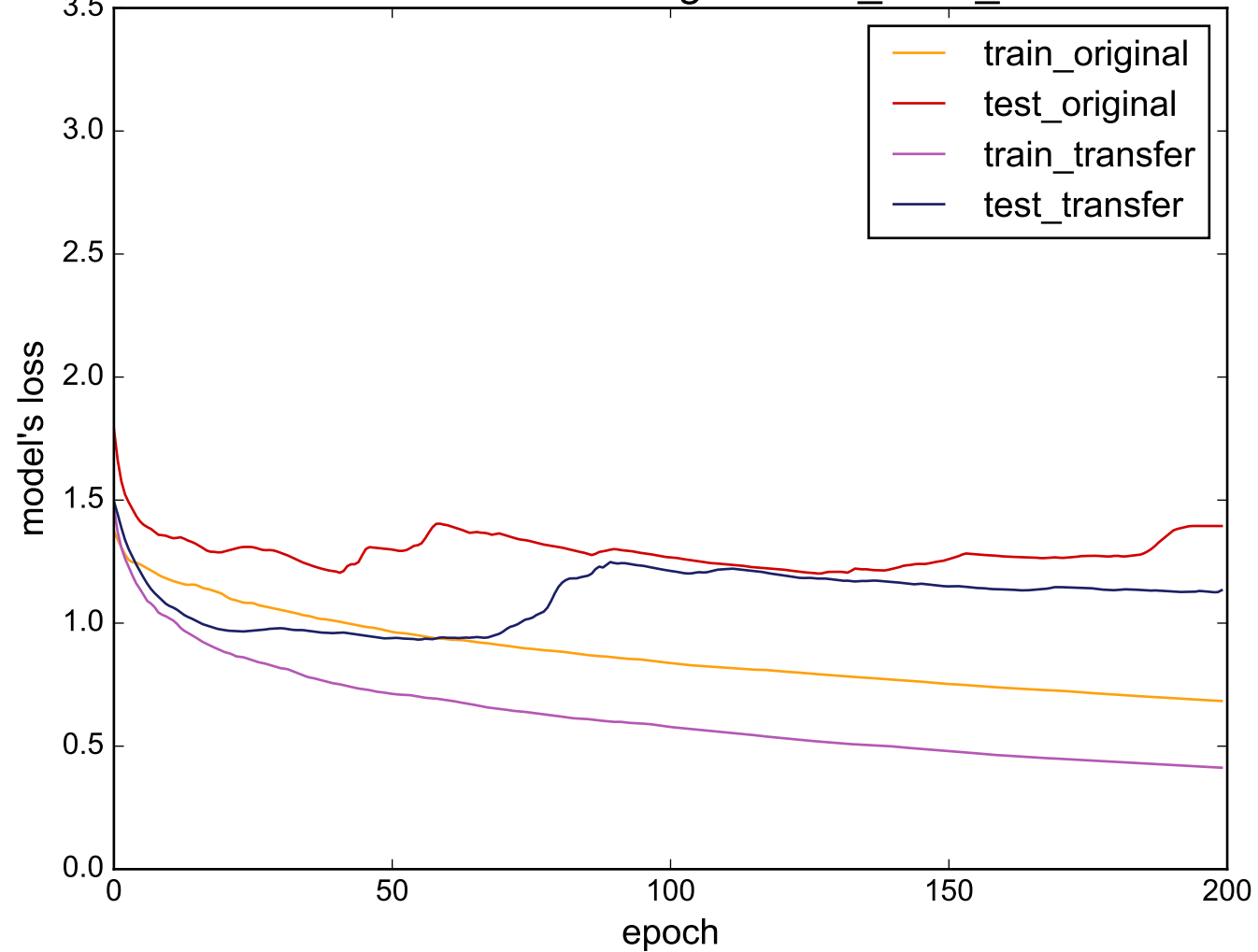
Source: MALLAT - Target: CinC_ECG_torso
