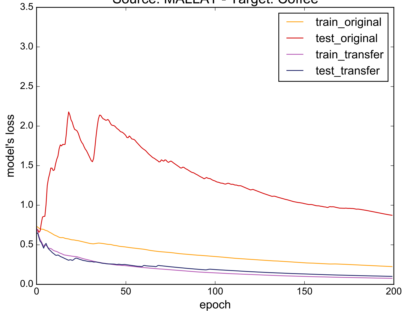
Source: MALLAT - Target: Coffee
