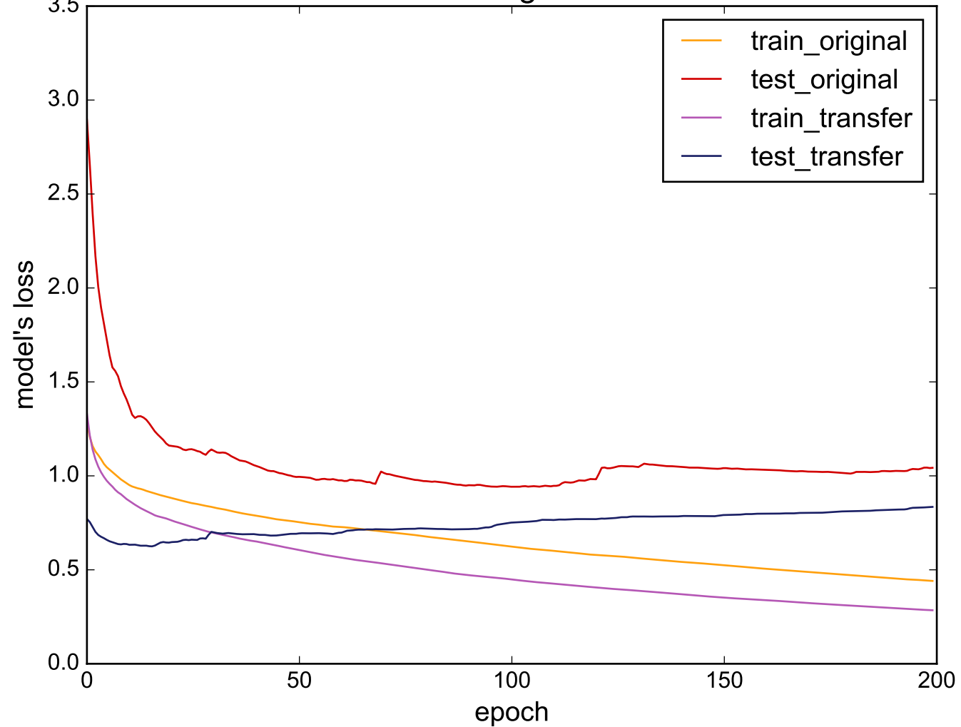
Source: MALLAT - Target: DistalPhalanxTW
