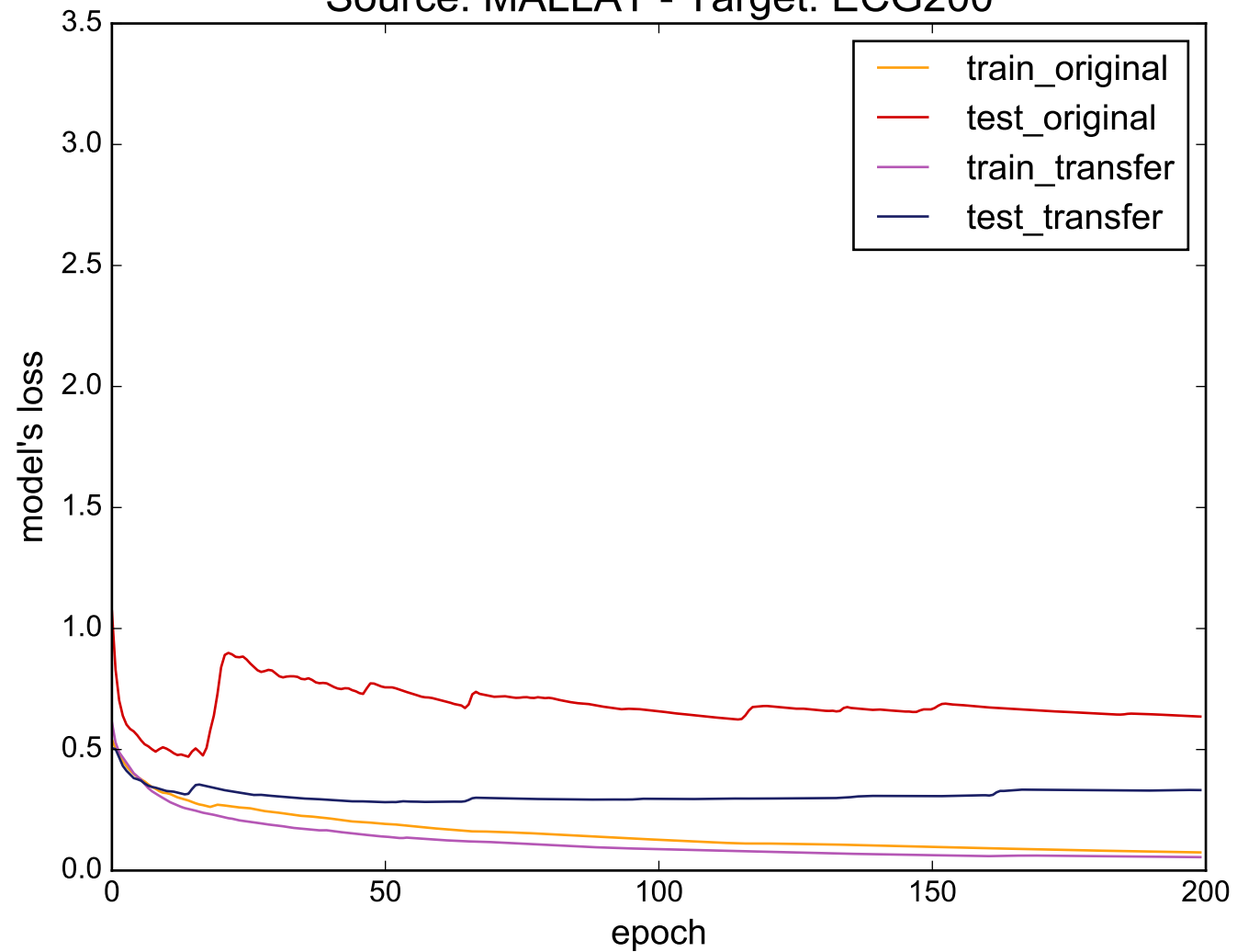
Source: MALLAT - Target: ECG200
