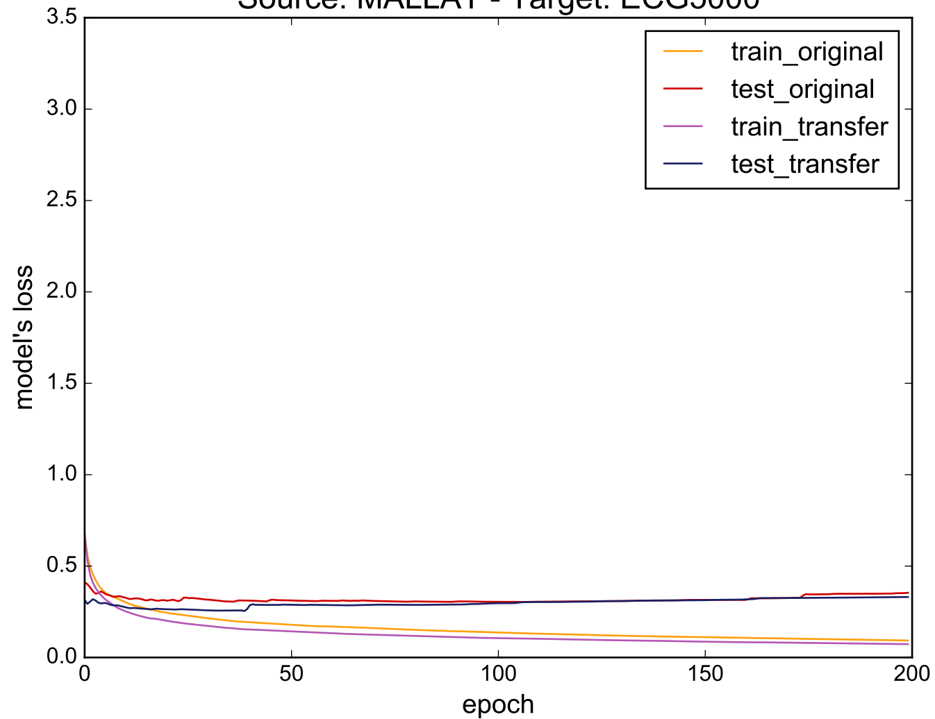
Source: MALLAT - Target: ECG5000
