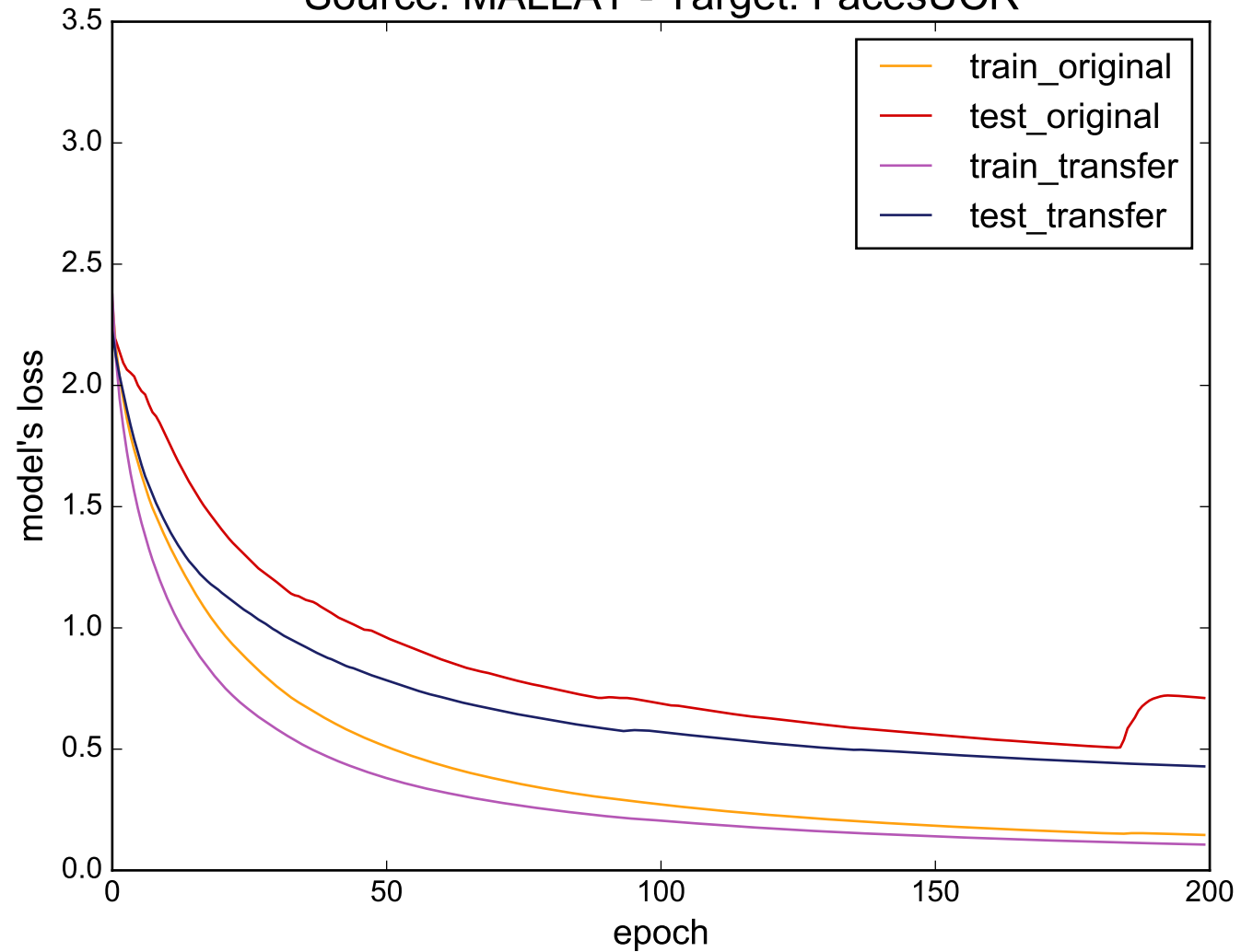
Source: MALLAT - Target: FacesUCR
